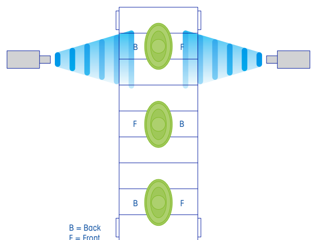
Above: An intelligent search system compensates for either front or back of bottle being presented to either camera.
